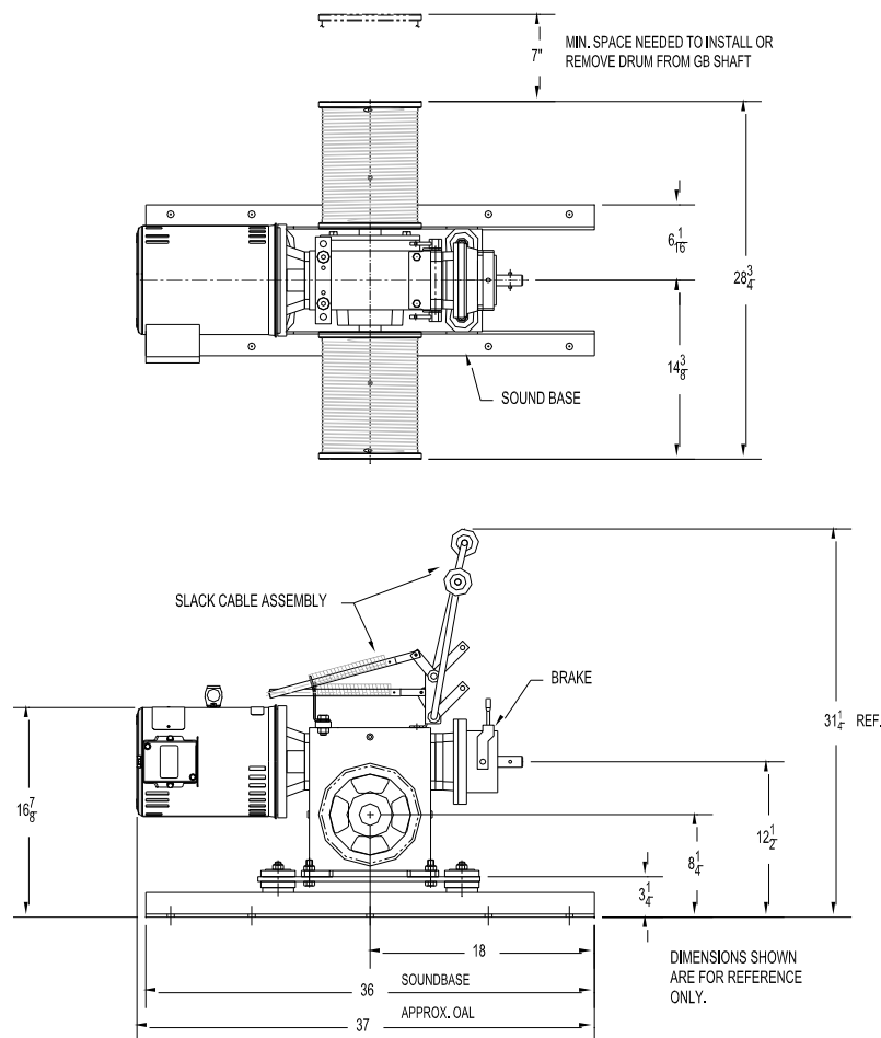
500# WD MACHINE - DOUBLE DRUM MOUNTED ON SOUND BASE
