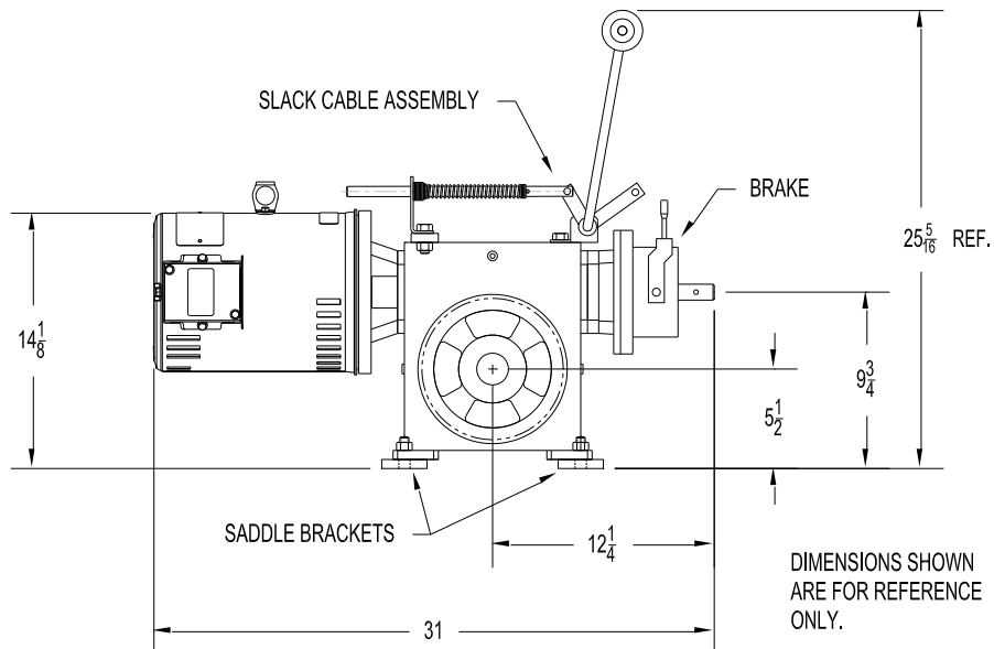
RH 500# WD MACHINE - SINGLE DRUM MOUNTED ON SADDLE BRACKETS
